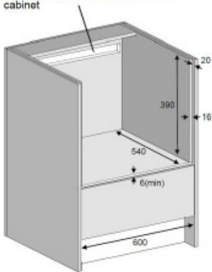
Ventilation: Option 1 Cutout 45mm x 500mm top rear of cabinet
