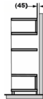
Ventilation: Option 3 (for tower installation) 45mm x cabinet width vented to top of cabinetry / into roof cavity.
